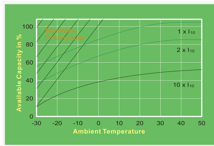
Extracted capacity in relation to the temperature.
